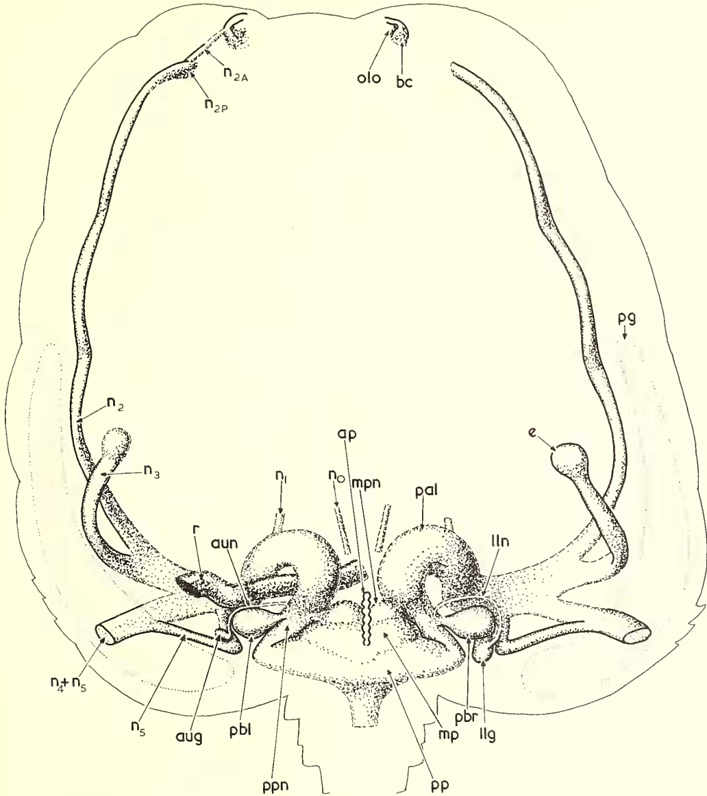
TEXT-FIG. 16. Reconstruction of brain and cranial nerves of Mitrocystites mitra in dorsal aspect (modified from Jefferies 1968, fig. 27). ap = anterior part of brain; aug = auditory ganglion; aun = auditory nerve; bc = buccal cavity; e = eye; llg = lateral line ganglion; lln = lateral line nerve; mp = medial part of brain; mpn = medial part nerve; n_0 = ventral nerves of uncertain connection and homology; n_{1-5} = nerves of palmar complex including maxillary trigeminal ( n_2 ) and optic ( n_3 ) nerves; n_{2A+P} = branches of nerve n_2 ; olo = olfactory openings; pal = palmar nerves; pbl and pbr = left and right pyramiform bodies (trigemino-profundus ganglia); pg = peripheral groove; pp = posterior part of brain; ppn = posterior part nerves; r = rectum.
